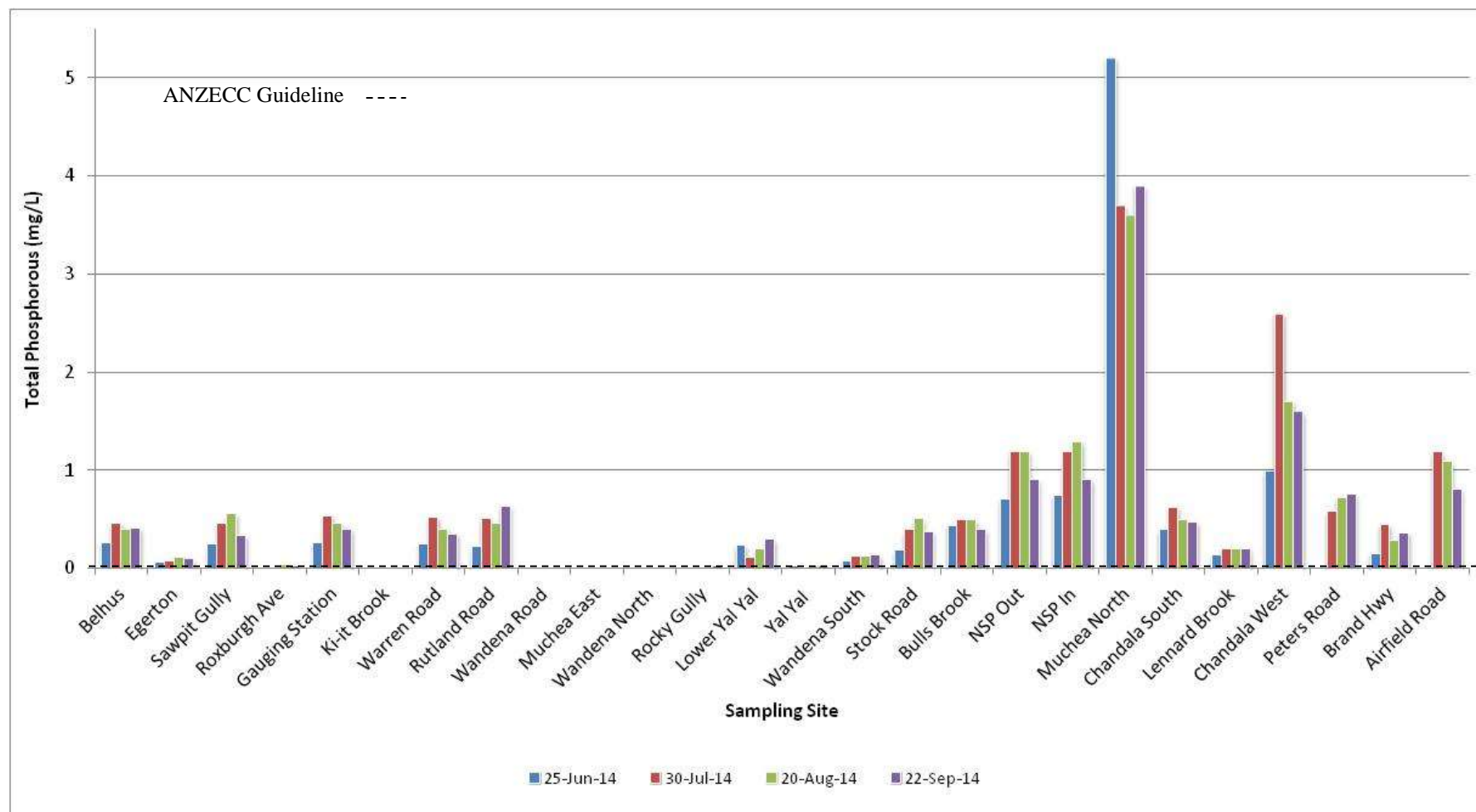
Figure 15: Total Phosphorous concentration sampled within the Ellen Brook catchment between June and September 2014.
