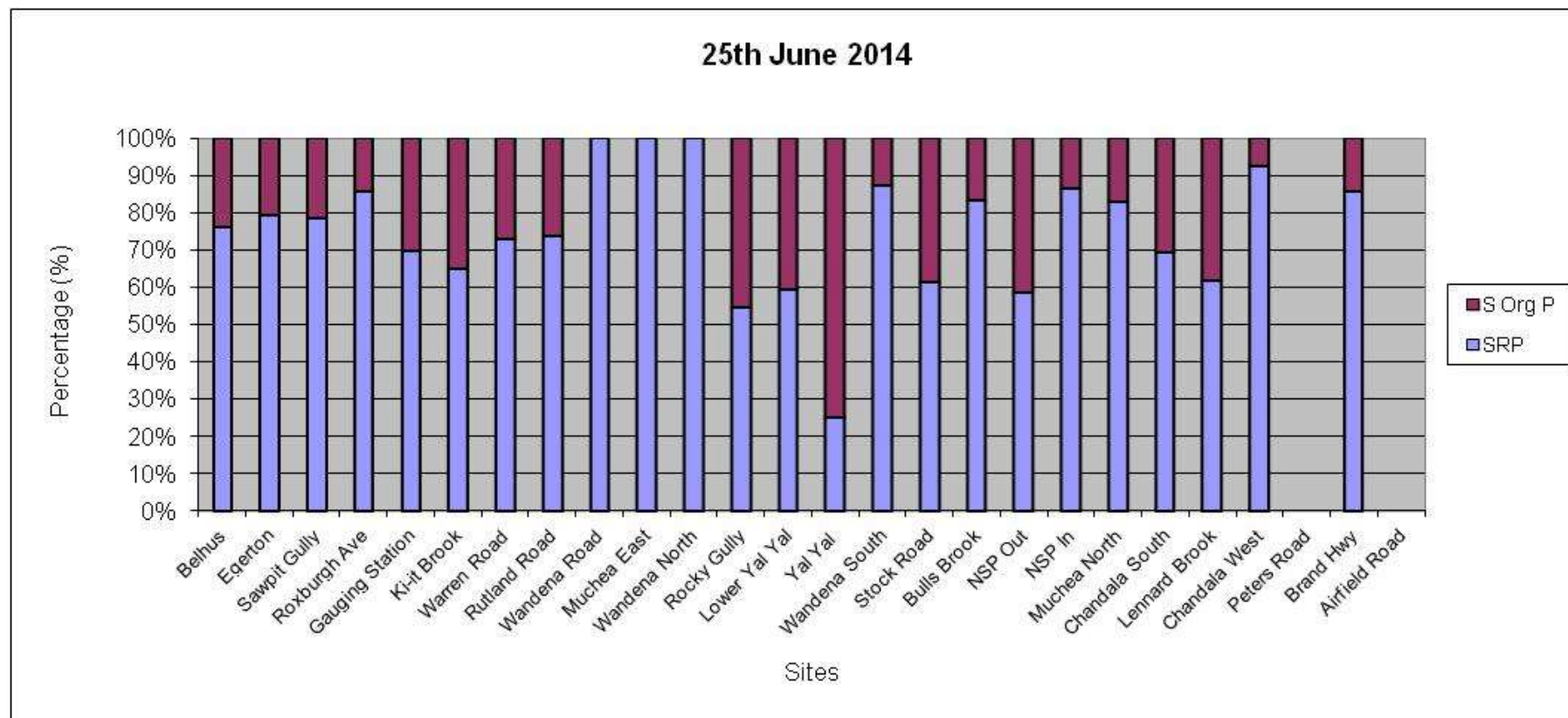
Figure 18: Composition of Total Filterable phosphorous in percentages of Soluble Organic P and SRP in June Sampling run 2014. *note that blanks represent no sample or TFP below LOR
