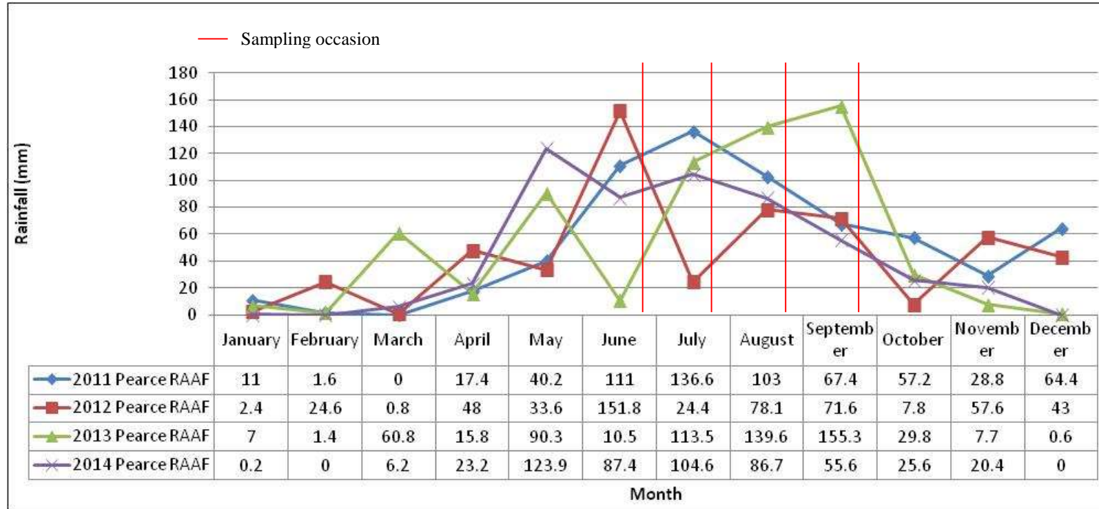
Figure 6: Total monthly rainfall for 2014, 2013, 2012 and 2011 within the Ellen Brook Catchment at 009053 – Pearce RAAF Base.
