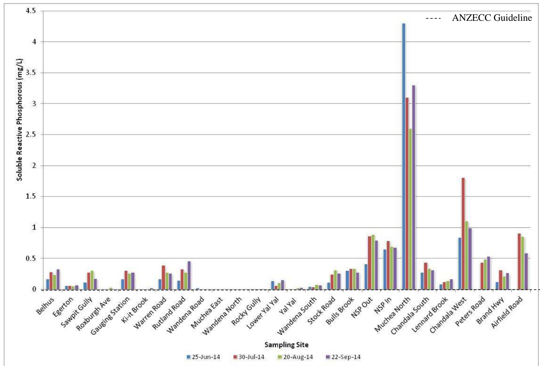
Figure 16: Soluble Reactive Phosphorous concentrations sampled within the Ellen Brook catchment between June and September 2014
