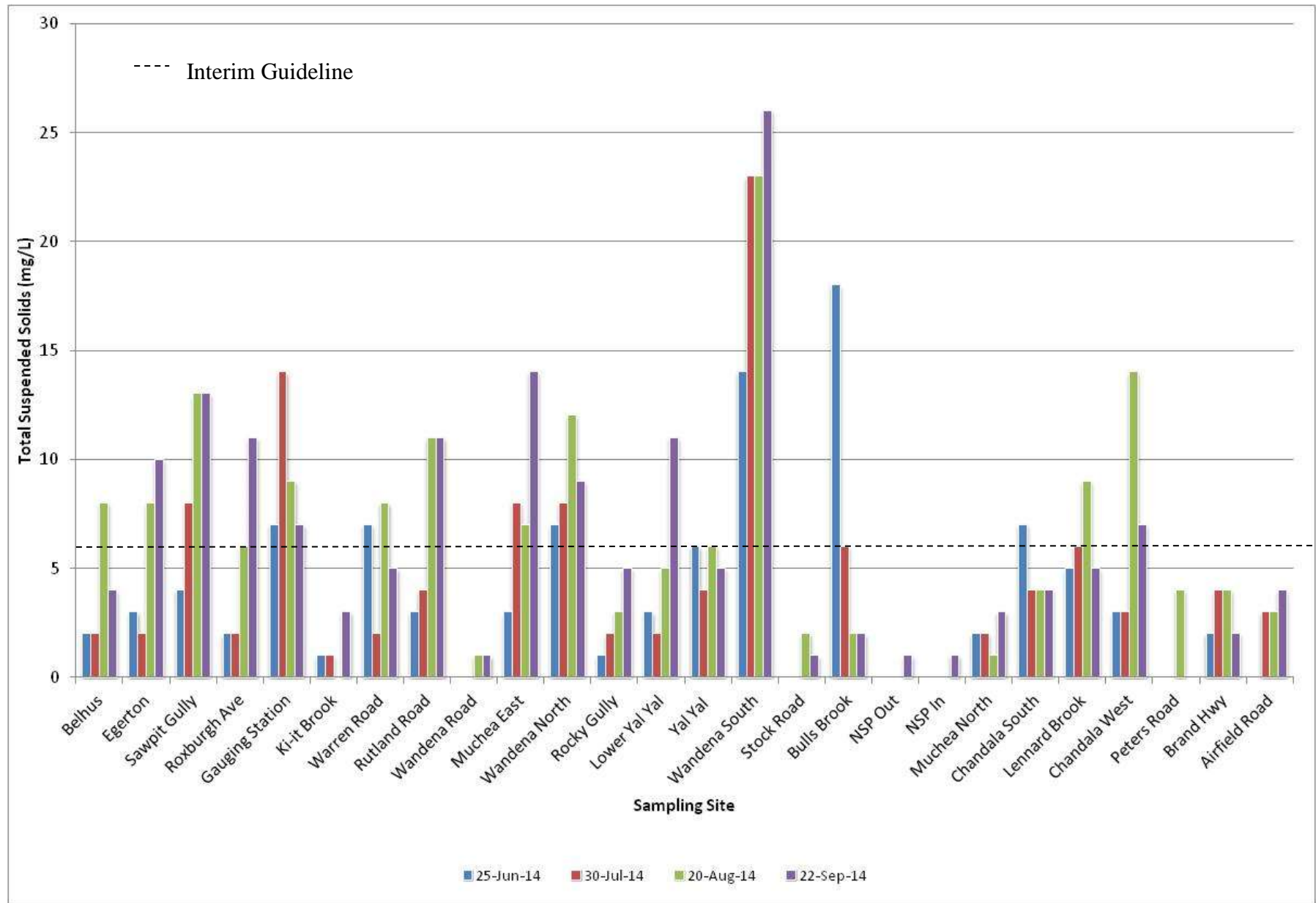
Figure 10: Total Suspended Solid concentrations in surface water within the Ellen Brook Catchment between June and September 2014. *Note blanks represent not sampled
