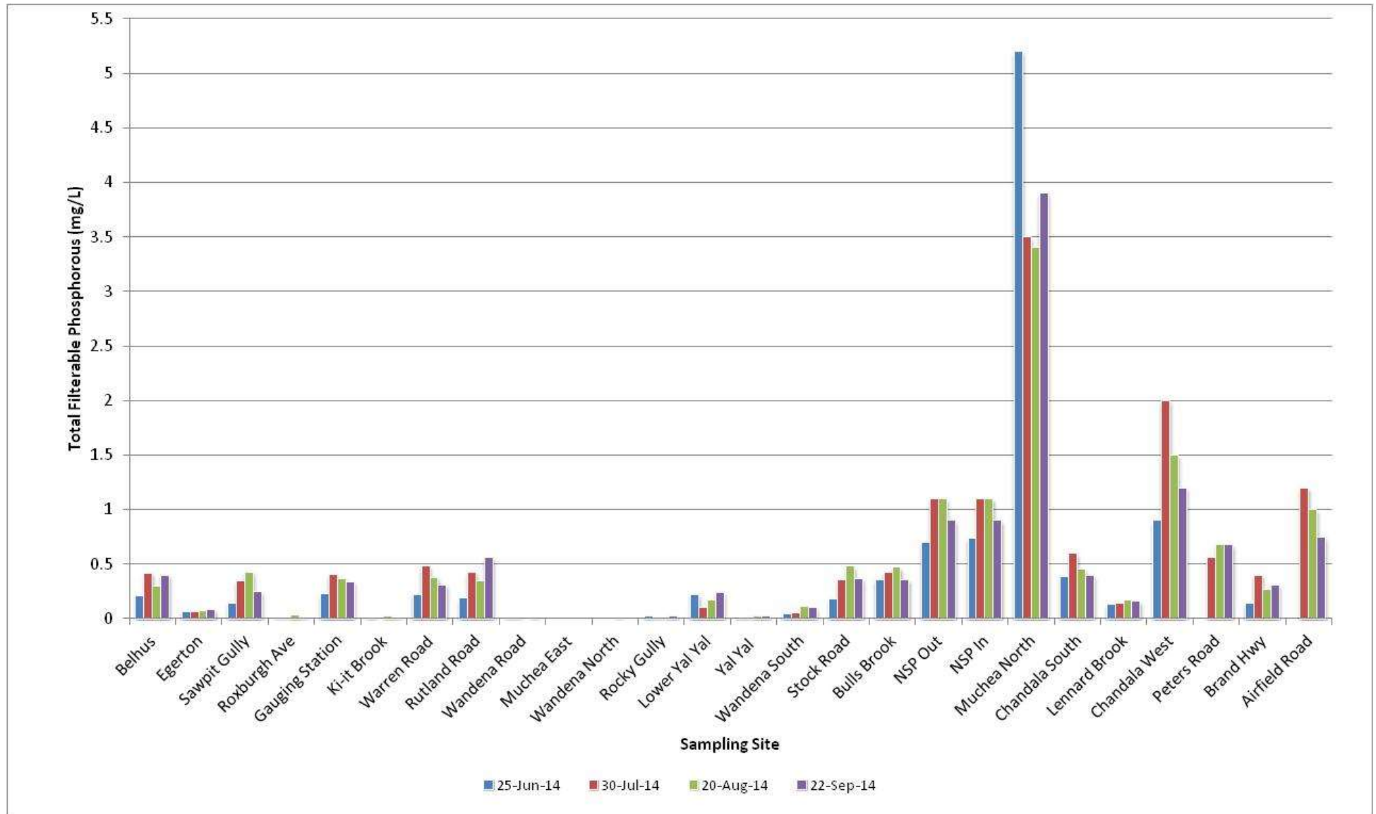
Figure 17: Total Filterable Phosphorous (TFP) concentrations sampled within the Ellen Brook catchment between June and September 2014.
