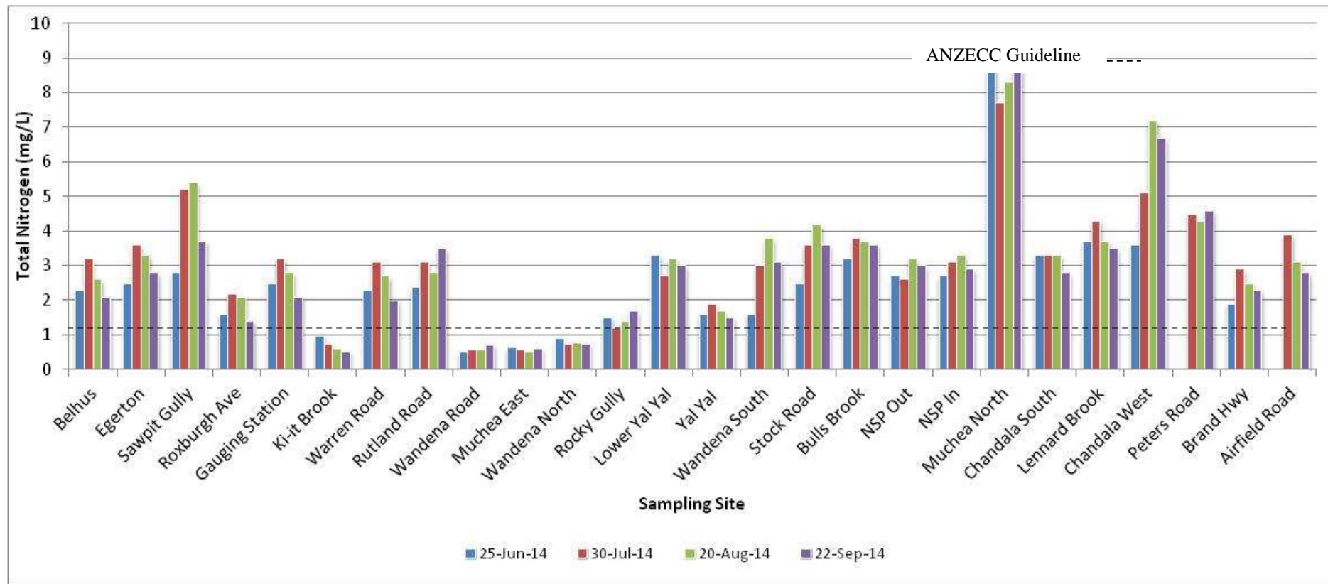
Figure 11: Total Nitrogen concentration in surface water within the Ellen Brook catchment sampled between June and September 2014.
