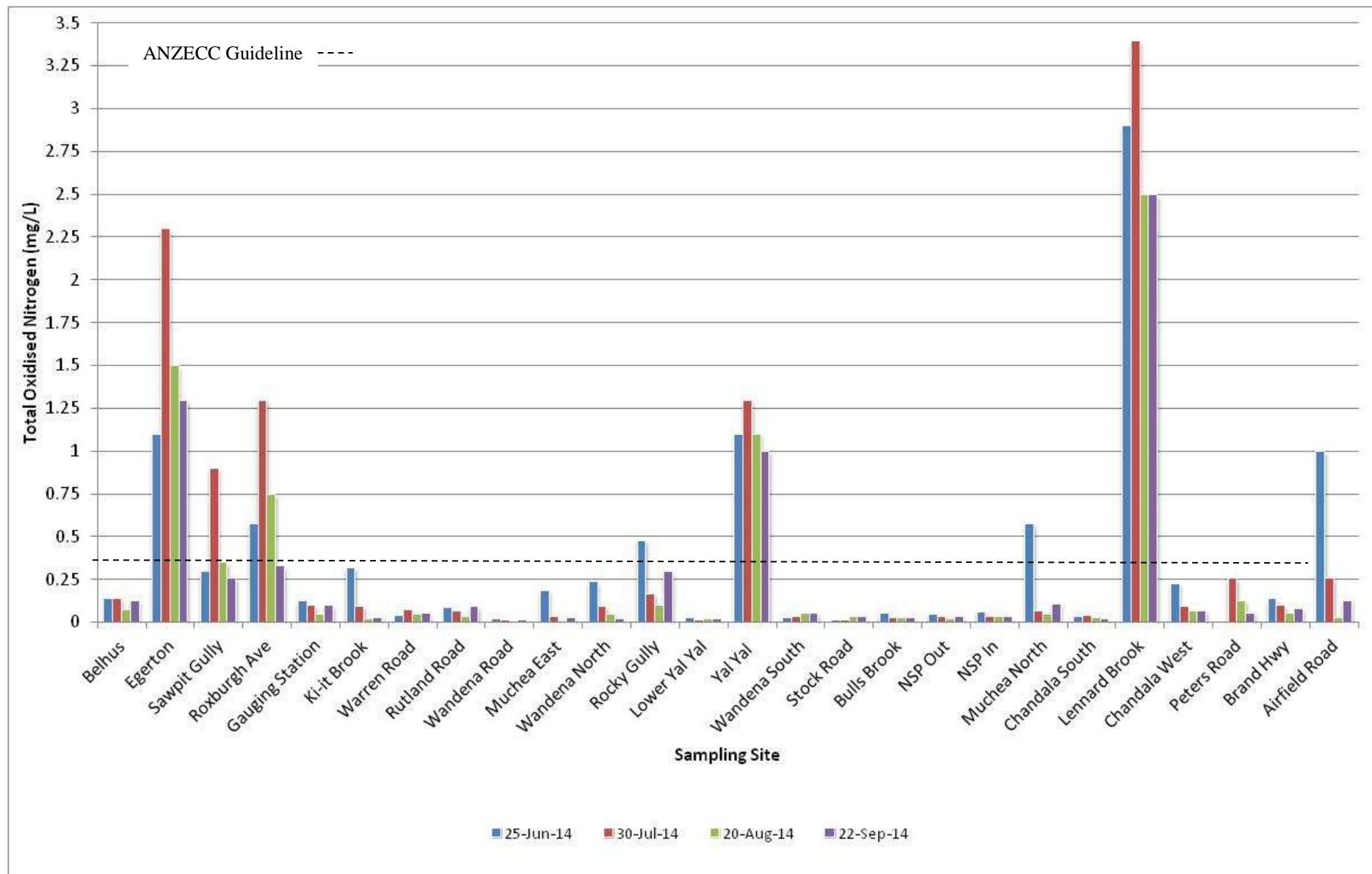
Figure 12: Total Oxidised Nitrogen (TON) sampled within the Ellen Brook catchment between June and September 2014. *Note blanks represent no sample.
