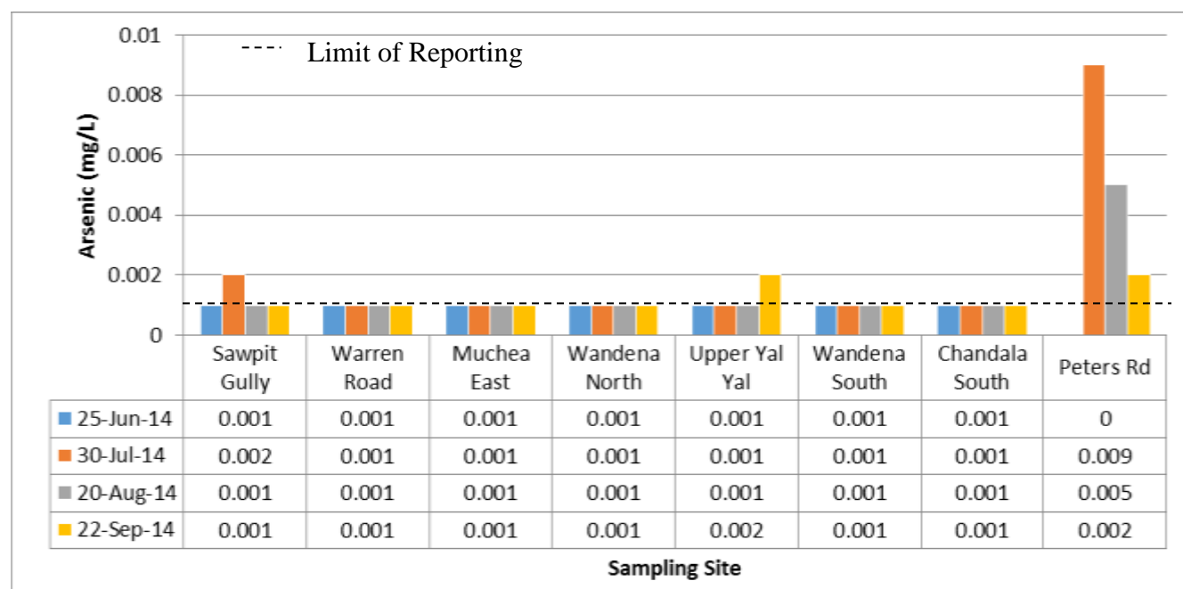
Figure 24: Arsenic concentrations in surface water within the Ellen Brook catchment between June and September 2014. *please note blanks represent no sample
