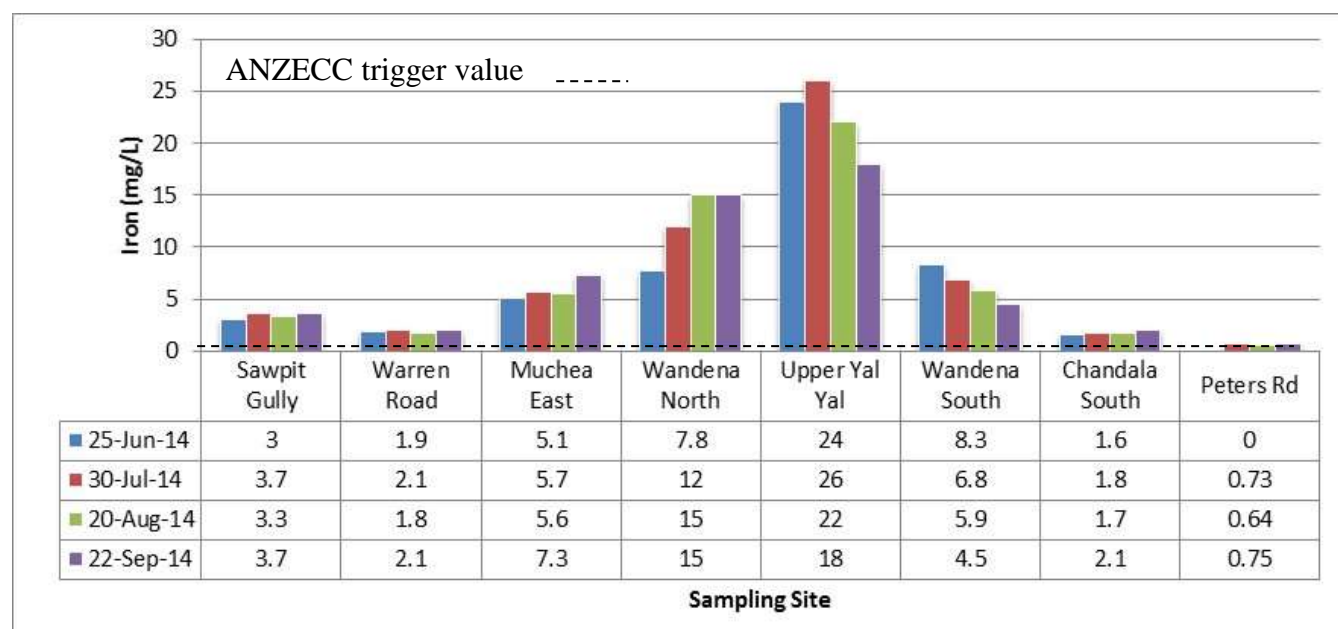
Figure 28: Iron concentrations in surface water within the Ellen Brook Catchment between June and September 2014. *please note blanks represent no sample
