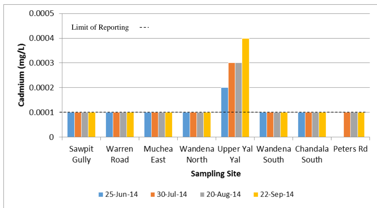
Figure 25: Cadmium concentrations in surface water within the Ellen Brook catchment between June and September 2014. *please note that blanks represent no sample
