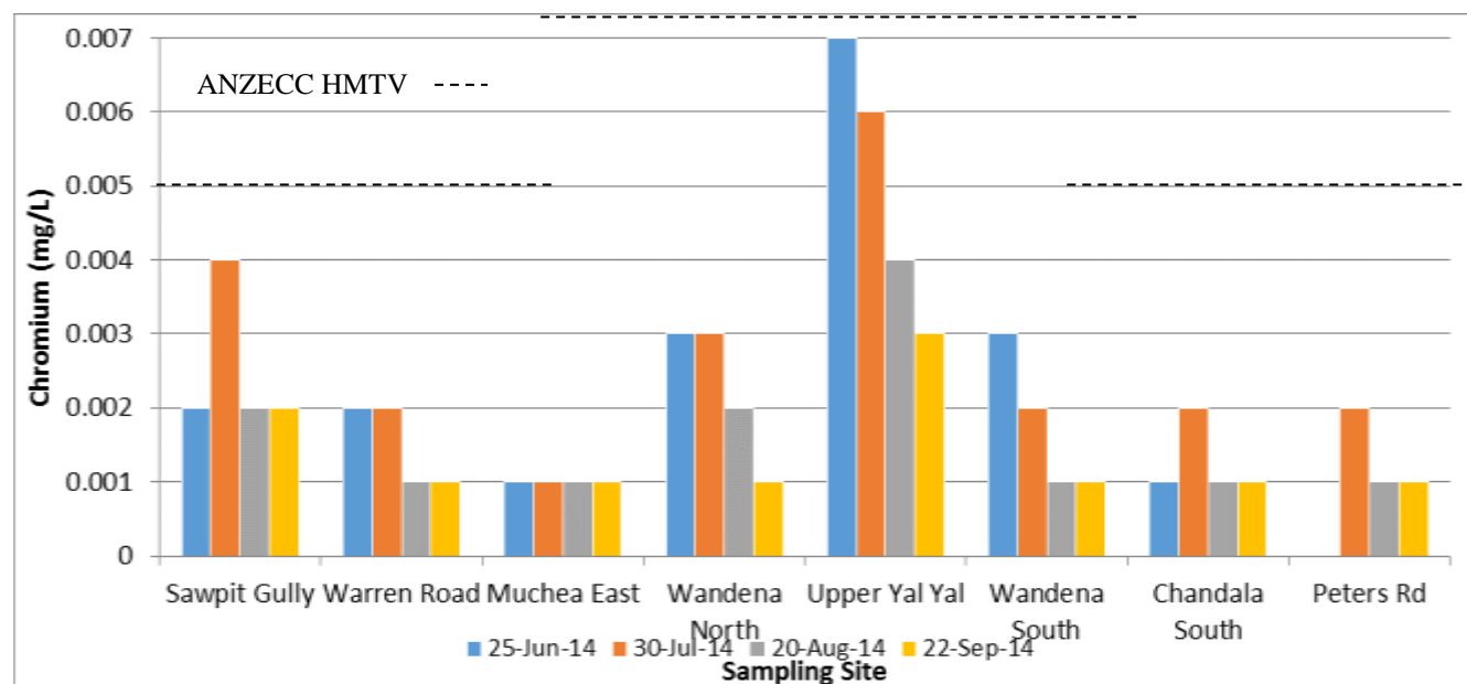
Figure 26: Chromium concentrations in surface water within the Ellen Brook catchment between June and September 2014. *Note blanks represent no sample.
