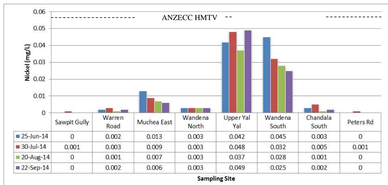
Figure 30: Nickel concentrations in surface water within the Ellen Brook catchment between June and September 2014. *Note blanks represent no sample
